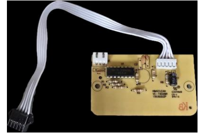
49-0001-66-6 PCB 2 EQUINOX
