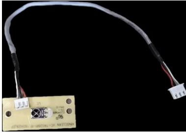
49-0001-65-7 PCB 1 EQUINOX
